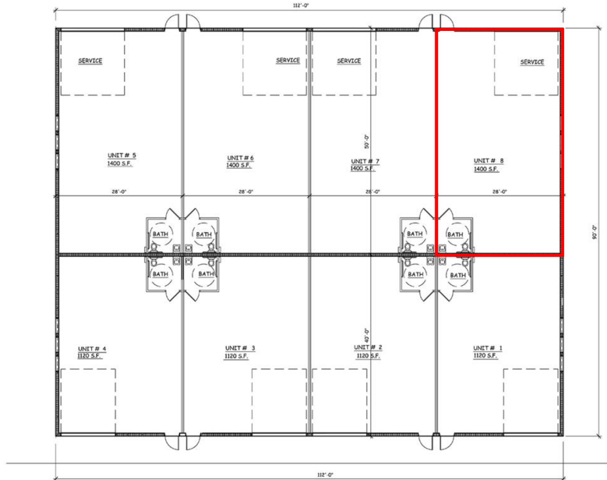
BUILDING 1 FLOOR PLAN 1/8"=1'-0"
