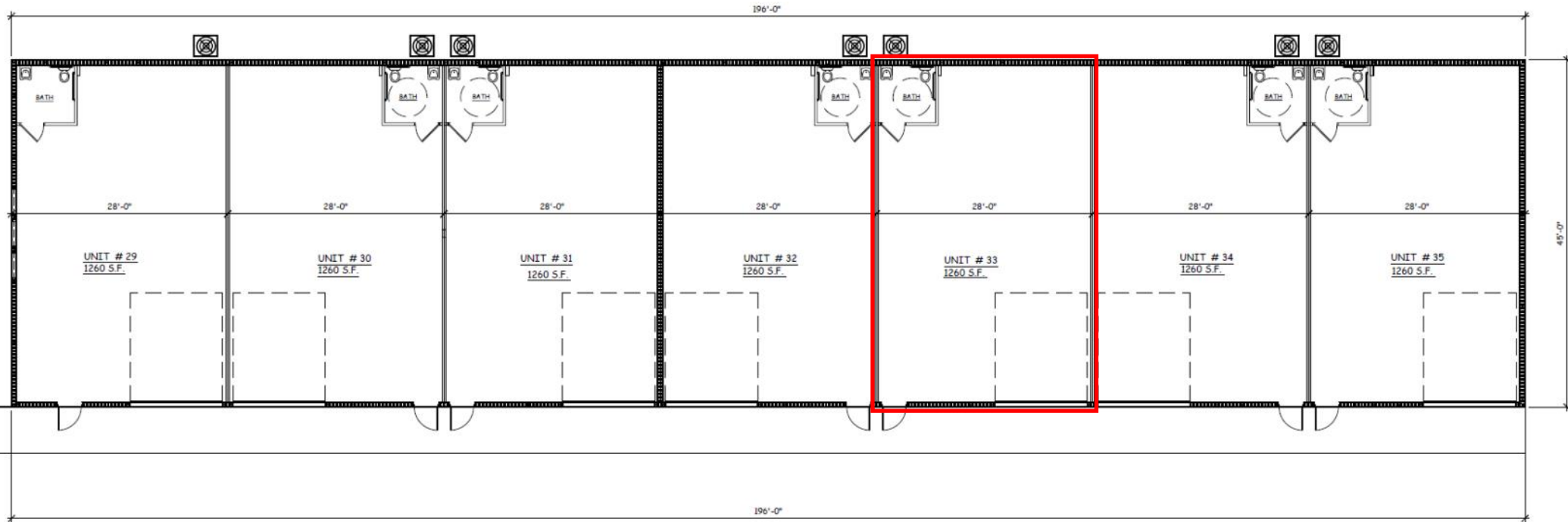
BUILDING 4 FLOOR PLAN 1/8"=1'-0"
