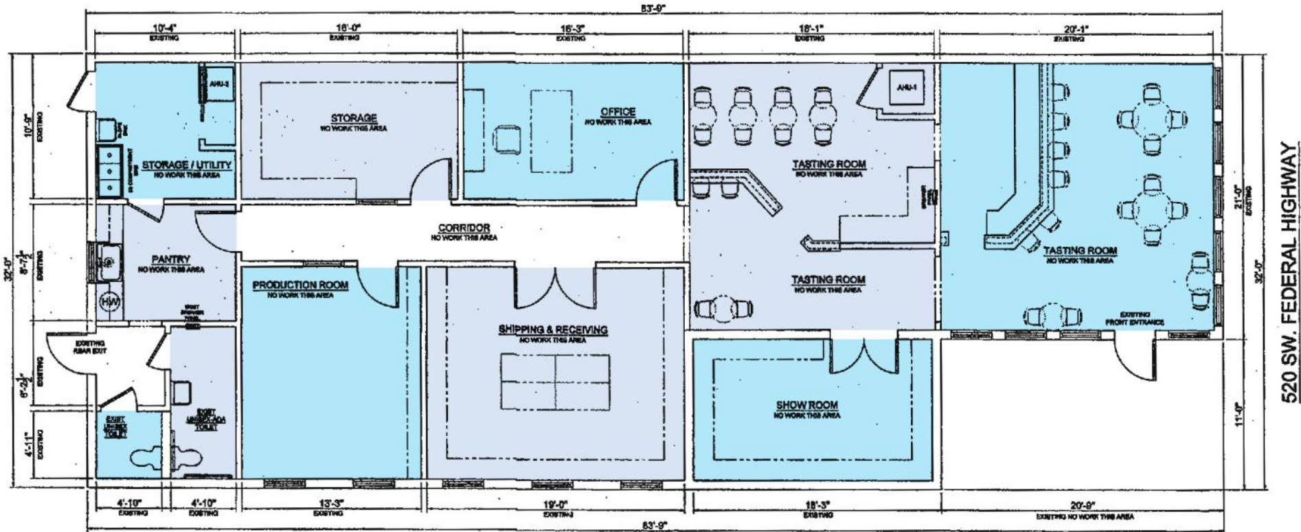
EXISTING FLOOR PLAN 1/4" = 1'-0"
